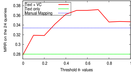
Fig. 3. MRR values on only 24 queries.
